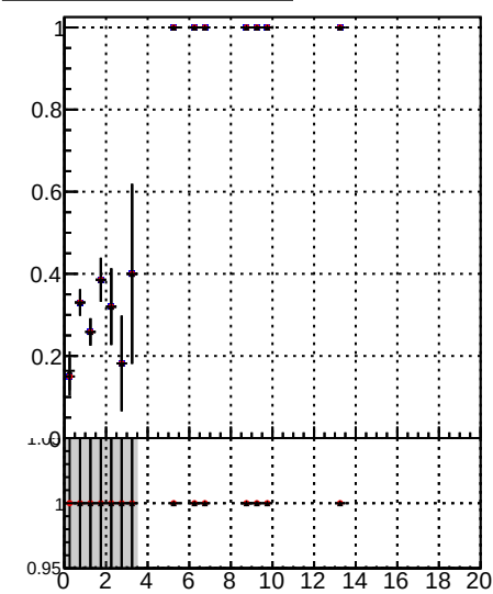
Fake rate vs. /data2/legianni/JSON-bkwd-fwd/no-modif/CMSSW_13_6_X_2023-01-24-1100/src/DQM_original BCM modified PL
