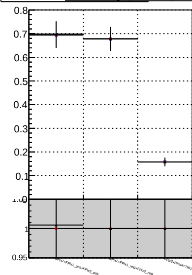
Fake rate vs. /data2/legianni/JSON-bkwd-fwd/no-modif/CMSSW_13_6_X_2023-01-24-1100/src/DQM_original BCM modified PL
