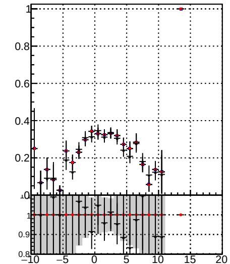
Fake rate vs. sim PV z
