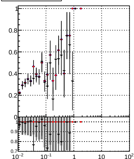
/data2/legianni/JSON-bkwd-fwd/no-modif/CMSSW_13_0_X_2023-01-24-1100/src/DQM_original Fake rate vs vertpos DQM_modified DQM_modified_PL
