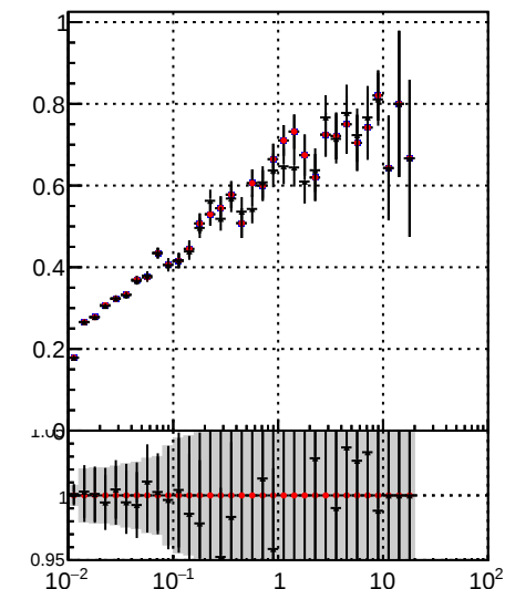
Fake rate vs v Legend: —•— /data2/legianni/JSON-bkwd-fwd/no-modif/CMSSW_13_0_X_2023-01-24-1100/src/DQM_original —•— DQM_modified —•— DQM_modified_PL
