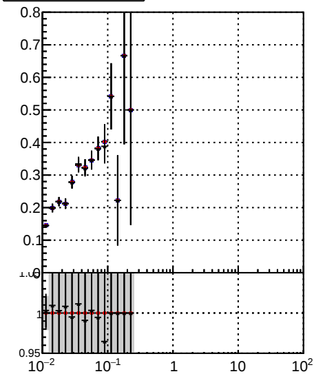
Fake rate vs verpos Legend: /data2/legianni/JSON-bkwd-fwd/no-modif/CMSSW_13_0_X_2023-01-24-1100/src/DQM_original DQM_modified DQM_modified_PL
