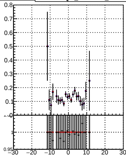
Fake rate vs vertpos Legend: /data2/legianni/JSON-bkwd-fwd/no-modif/CMSSW_13_0_X_2023-01-24-1100/src/DQM_original DQM_modified DQM_modified_PL
