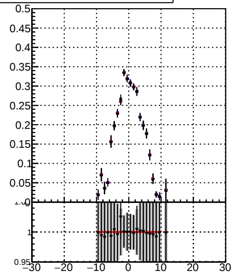
/data2/legianni/JSON-bkwd-fwd/no-modif/CMSSW_13_0_X_2023-01-24-1100/src/DQM_original Fake rate vs verpos, Duplicates Rate vs verpos, Pileup rate vs verpos
