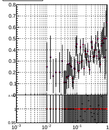
/data2/legianni/JSON-bkwd-fwd/no-modif/CMSSW_13_0_X_2023-01-24-1100/src/DQM_original Fake rate vs dr DQM_modified DQM_modified_PL
