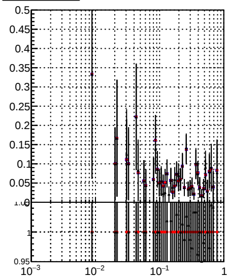
/data2/legianni/JSON-bkwd-fwd/no-modif/CMSSW_13_0_X_2023-01-24-1100/src/DQM_original Fake rate vs dr DQM_modified DQM_modified_PL
