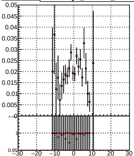
Fake rate vs vertpos Legend: /data2/legianni/JSON-bkwd-fwd/no-modif/CMSSW_13_0_X_2023-01-24-1100/src/DQM_original (black), DQM_modified (red), DQM_modified_PL (grey)
