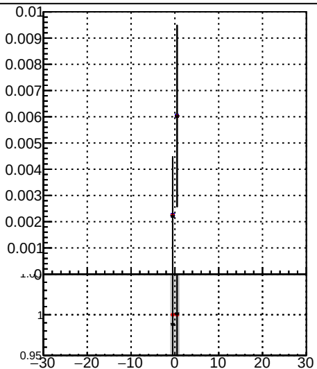
Fake rate vs vertpos - /data2/legianni/JSON-bkwd-fwd/no-modif/CMSSW_13_0_X_2023-01-24-1100/src/DQM_original - DQM_modified - DQM_modified_PL
