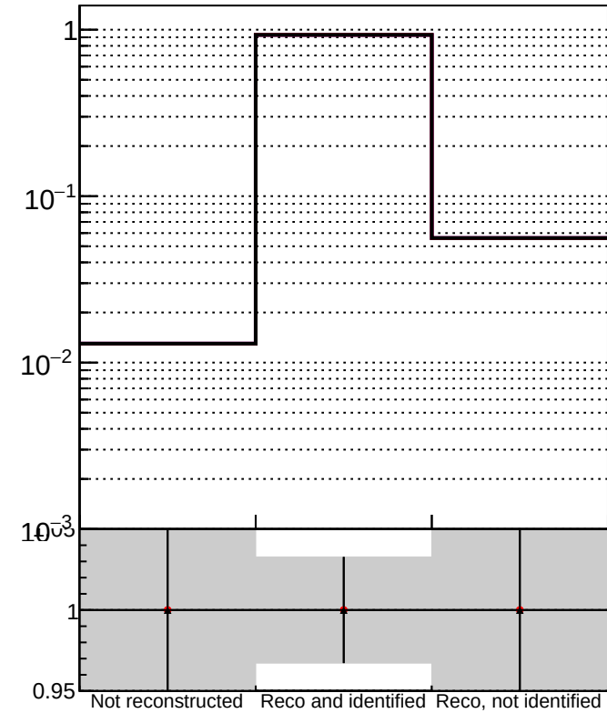
TruePVLocationIndexInRecoVertexCollectionCumulative
