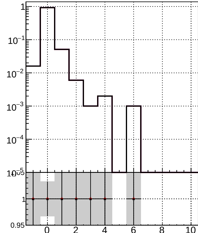
TruePVLocationIndexInRecoVertexCollection
