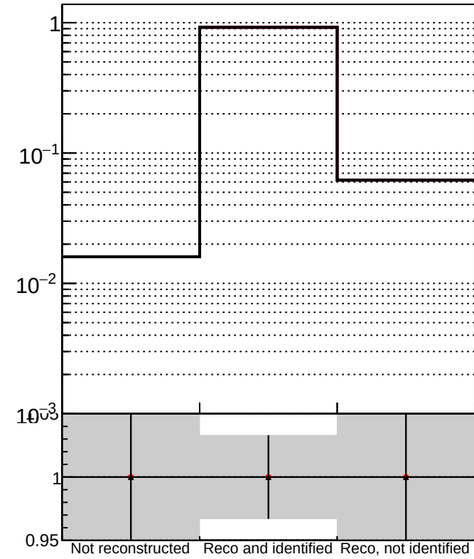
TruePVLocationIndexInRecoVertexCollectionCumulative
