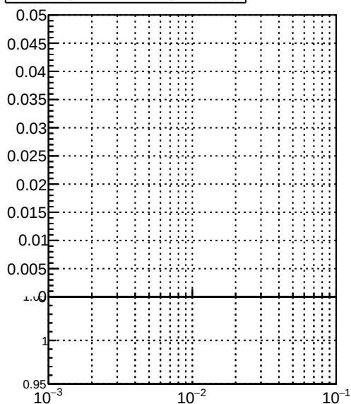
fake+duplicates vs \Delta R (track, jet)
