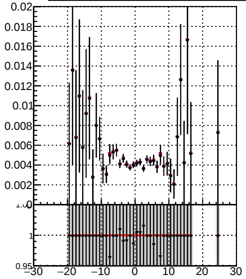
Efficiency vs vertpos Legend: \bullet /data2/legianni/JSON-bkwd-fwd/no-modif/CMSSW_13_0_X_2023-01-24-1100/src/DQM_original \bullet DQM_modified \bullet DQM_modified_PL
