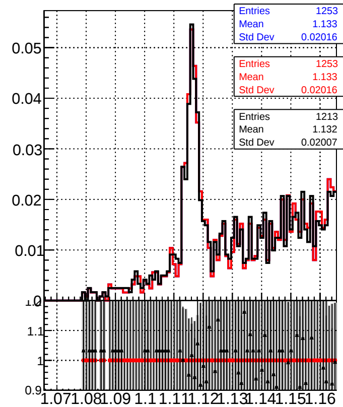
Invariant mass of all \Lambda^0
