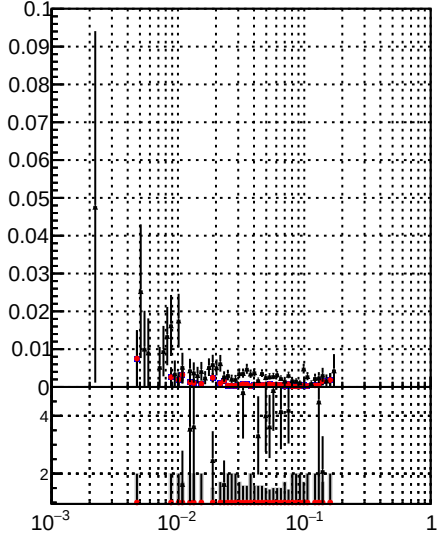
Legend: /data2/legianni/JSON-bkwd-fwd/no-modif/CMSSW_13_0_X_2023-01-24-1100/src/DQM_original (grey line with dots), DQM_modified (red line with diamonds), DQM_modified_PL (black line with crosses)
