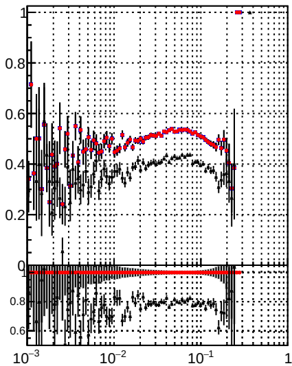
Legend: /data2/legianni/JSON-bkwd-fwd/no-modif/CMSSW_13_0_X_2023-01-24-1100/src/DQM_original (grey line with dots), DQM_modified (red line with diamonds), DQM_modified_PL (black line with crosses)
