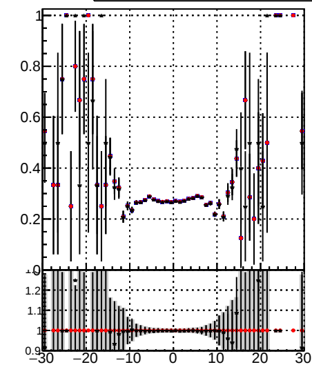
Legend: /data2/legianni/JSON-bkwd-fwd/no-modif/CMSSW_13_0_X_2023-01-24-1100/src/DQM_original (black squares), DQM_modified (red circles), DQM_modified_PL (black crosses)
