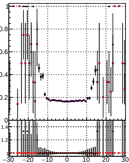
/data2/legianni/JSON-bkwd-fwd/no-modif/CMSSW_13_0_X_2023-01-24-1100/src/DQM_original Fake rate vs v DQM_modified DQM_modified_PL
