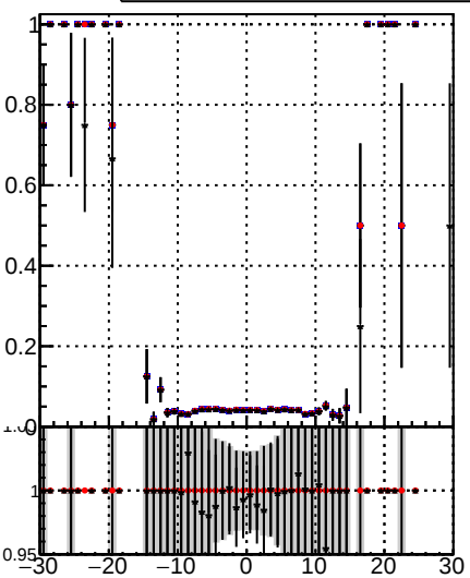
/data2/legianni/JSON-bkwd-fwd/no-modif/CMSSW_13_0_X_2023-01-24-1100/src/DQM_original Fake rate vs vertpos DQM_modified DQM_modified_PL
