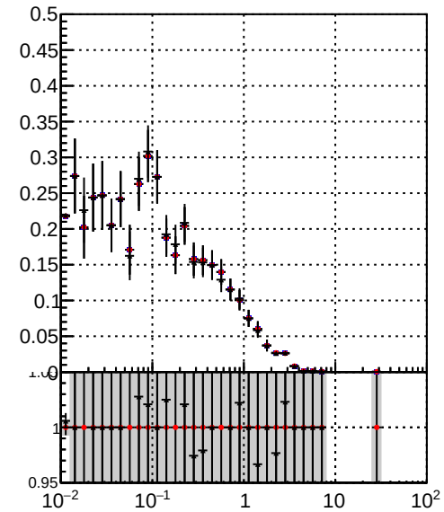
Efficiency vs vertpos Legend: — /data2/legianni/JSON-bkwd-fwd/no-modif/CMSSW_13_0_X_2023-01-24-1100/src/DQM_original — DQM_modified — DQM_modified_4iter-NewERR
