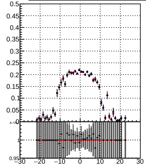
Efficiency vs vertpos Legend: — /data2/legianni/JSON-bkwd-fwd/no-modif/CMSSW_13_0_X_2023-01-24-1100/src/DQM_original — DQM_modified — DQM_modified_4iter-NewERR
