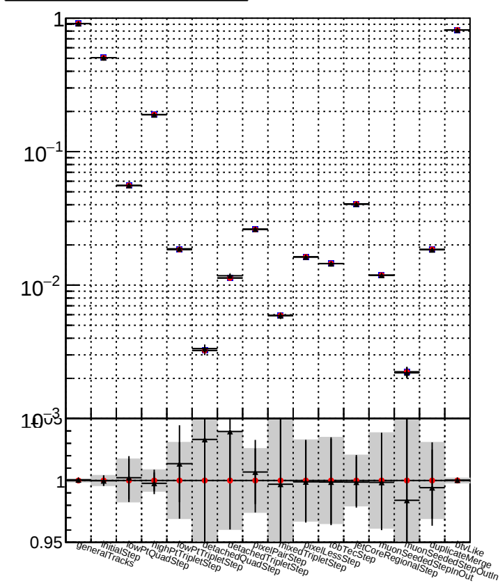
Duplicates rate vs collection Legend: /data2/legianni/JSON-bkwd-fwd/no-modif/CMSW_13_0_X_2023-01-24-1100/src/DQM_original DQM_modified DQM_modified_4iter-NewERR
