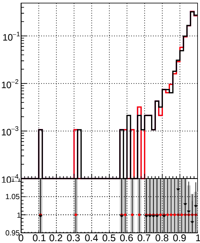
RecoPVAssoc2GenPVMatched_Purity
