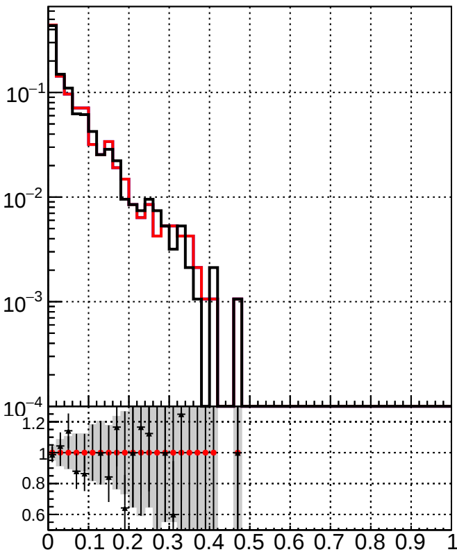
RecoPVAssoc2GenPVMatched_Missing
