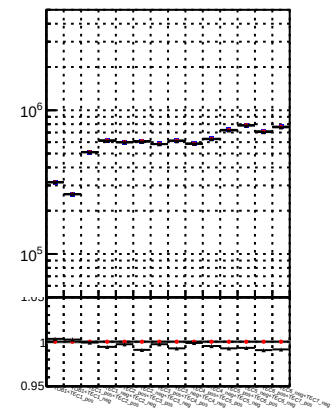
N of reco track vs. \chi^2 (data2legion/JSON-bkwd-fwd/no-modif/CMSSW_13_0_X_2023-01-24-1100/src/DQM-original)
