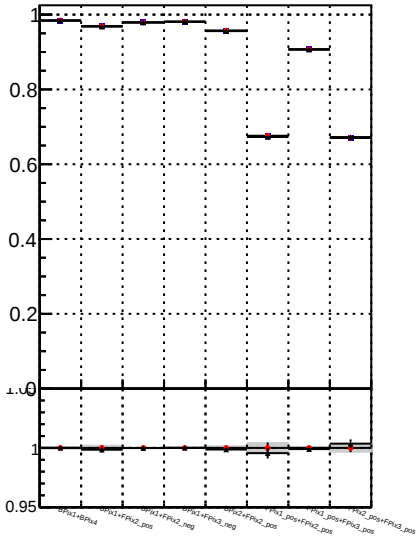
Fake rate vs. /data2/legianni/JSON-bkwd-fwd/no-modif/CMSSW_13_6_X_2023-01-24-1100/src/DQM_original BQM modified 4iter-NewERR BQM modified 4iter-NewERR
