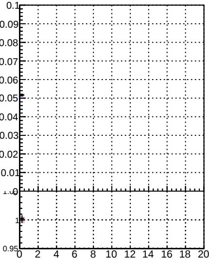
Fake rate vs. /data2/legianni/JSON-bkwd-fwd/no-modif/CMSSW_13_6_X_2023-01-24-1100/src/DQM_original BQM modified 4iter-NewERR BQM modified 4iter-NewERR
