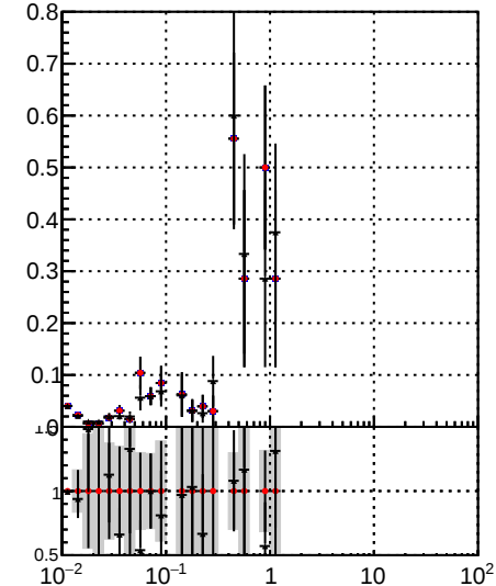
Legend: /data2/legianni/JSON-bkwd-fwd/no-modif/CMSSW_13_0_X_2023-01-24-1100/src/DQM_original (black circles), DQM_modified (red circles), DQM_modified_4iter-NewERR (black circles with error bars)
