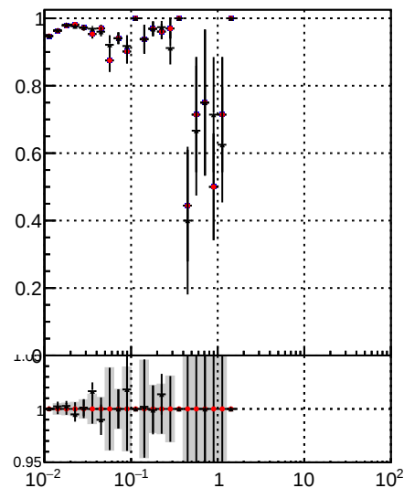
Legend: /data2/legianni/JSON-bkwd-fwd/no-modif/CMSSW_13_0_X_2023-01-24-1100/src/DQM_original (black circles), DQM_modified (red circles), DQM_modified_4iter-NewERR (black circles with error bars)
