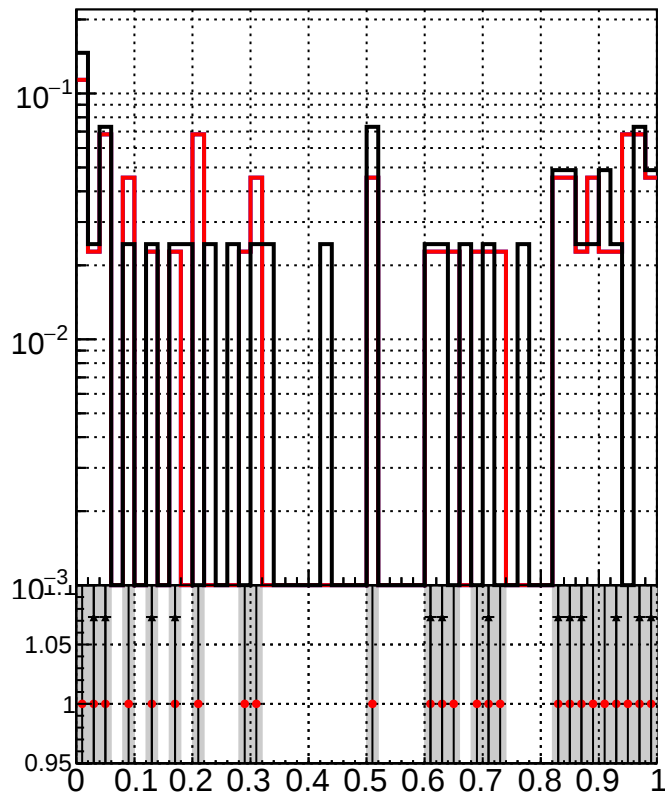
RecoPVAssoc2GenPVNotMatched_Missing
