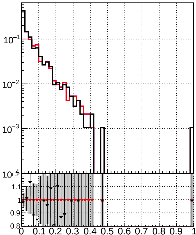
RecoPVAssoc2GenPVMatched_Missing
