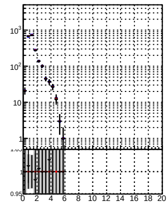
N of reco track vs. \chi^2 for data2/legionmi/JSON-bkwd-fwd/no-modif/CMSSW_13_0_X_2023-01-24-1100/src/DQM-original, DQM modified 4iter-NewERR, and DQM modified 4iter-NewERR
