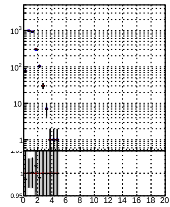
N of reco track vs. \chi^2 for \sqrt{s}=13 TeV, 36.1 fb ^{-1} data, 4iter-NewER, JSON-bkwd-fwd/no-modif/CMSSW_13_0_X_2023-01-24-1100/src/DQM-original
