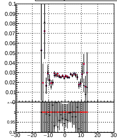
/data2/legianni/JSON-bkwd-fwd/no-modif/CMSSW_13_0_X_2023-01-24-1100/src/DQM_original DQM_modified DQM_modified_4iter-NewERR Fake rate vs v
