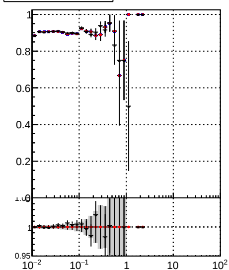
/data2/legianni/JSON-bkwd-fwd/no-modif/CMSSW_13_0_X_2023-01-24-1100/src/DQM_original DQM_modified DQM_modified_4iter-NewERR Fake rate vs v
