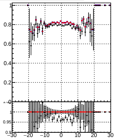
Legend: /data2/legianni/JSON-bkwd-fwd/no-modif/CMSSW_13_0_X_2023-01-24-1100/src/DQM_original (black circles), DQM_modified (red circles), DQM_modified_4iter-NewERR (black crosses)
