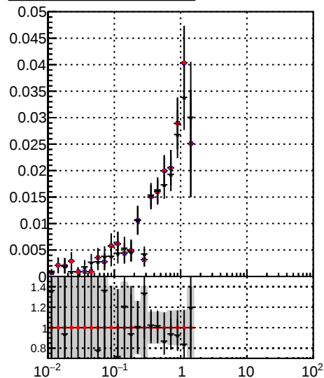
Legend: /data2/legianni/JSON-bkwd-fwd/no-modif/CMSSW_13_0_X_2023-01-24-1100/src/DQM_original (black circles), DQM_modified (red circles), DQM_modified_4iter-NewERR (black crosses)
