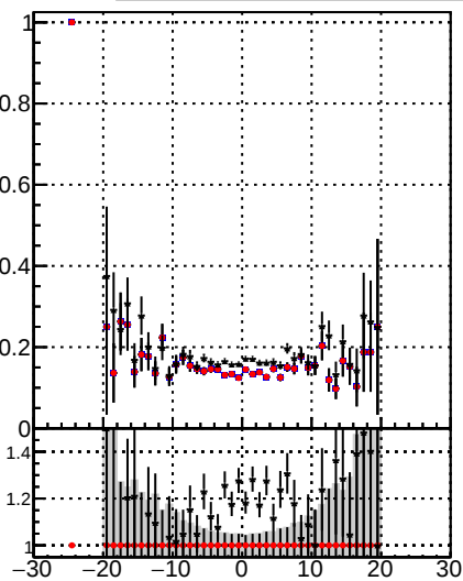
Legend: /data2/legianni/JSON-bkwd-fwd/no-modif/CMSSW_13_0_X_2023-01-24-1100/src/DQM_original (black circles), DQM_modified (red circles), DQM_modified_4iter-NewERR (black crosses)
