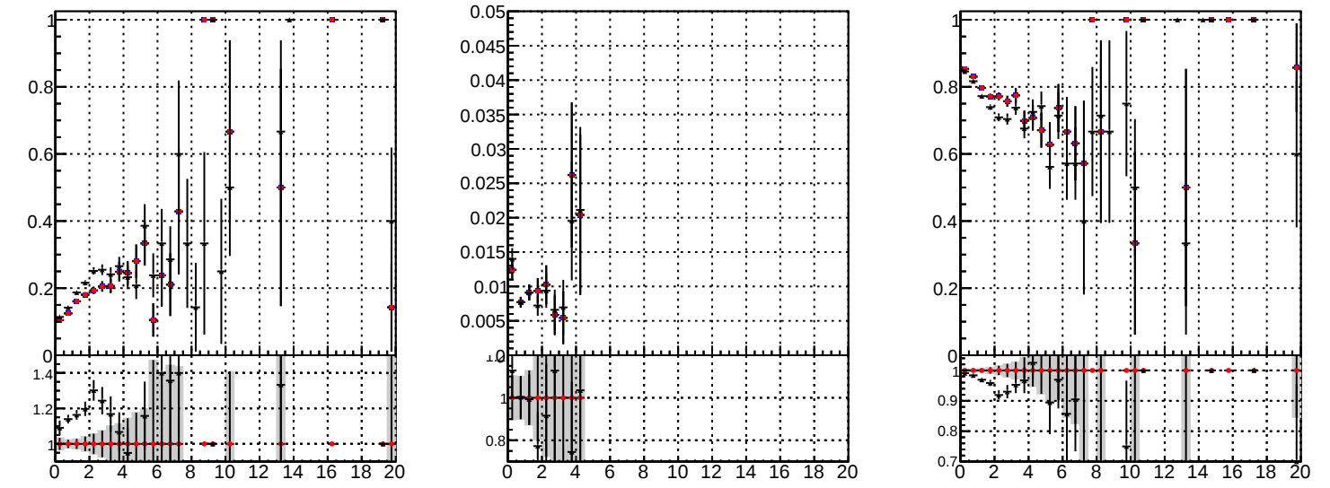
Fake rate vs. /data2/legianni/JSON-bkwd-fwd/no-modif/CMSSW_13_0_X_2023-01-24-1100/src/DQM_original BQM modified 4iter-NewERR
