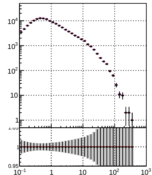
N of simulated tracks vs pT
