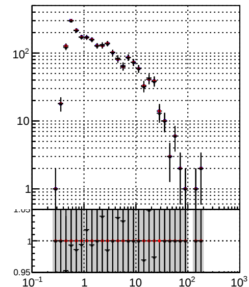
N of associated tracks (simToReco) vs pT
