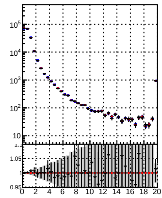
N of reco track vs. \chi^2 data2/legsim/JSON-bkwd-fwd/no-modif/CMSSW_13_0_X_2023-01-24-1100/src/DQM_original DQM modified 4iter-NewERR
