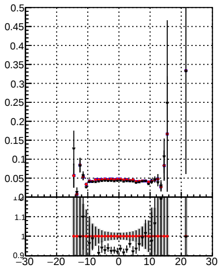
/data2/legianni/JSON-bkwd-fwd/no-modif/CMSSW_13_6_X_2023-01-24-1100/src/DQM_original Fake rate vs d BQM modified 4iter-NewERR
