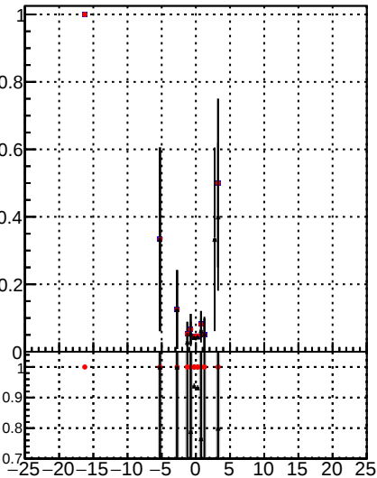
/data2/legianni/JSON-bkwd-fwd/no-modif/CMSSW_13_6_X_2023-01-24-1100/src/DQM_original Fake rate vs d BQM modified 4iter-NewERR
