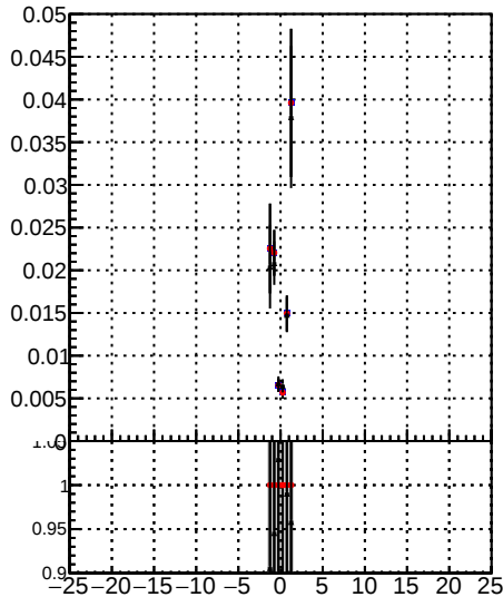
/data2/legianni/JSON-bkwd-fwd/no-modif/CMSSW_13_6_X_2023-01-24-1100/src/DQM_original Fake rate vs d BQM modified 4iter-NewERR
