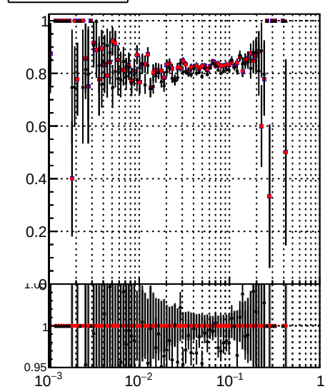
/data2/legianni/JSON-bkwd-fwd/no-modif/CMSSW_13_0_X_2023-01-24-1100/src/DQM_original DQM_modified DQM_modified_4iter-NewERR
