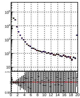
N of reco track vs. \chi^2 for data2/legsim/JSON-bkwd-fwd/no-modif/CMSSW_13_0_X_2023-01-24-1100/src/DQM-original
