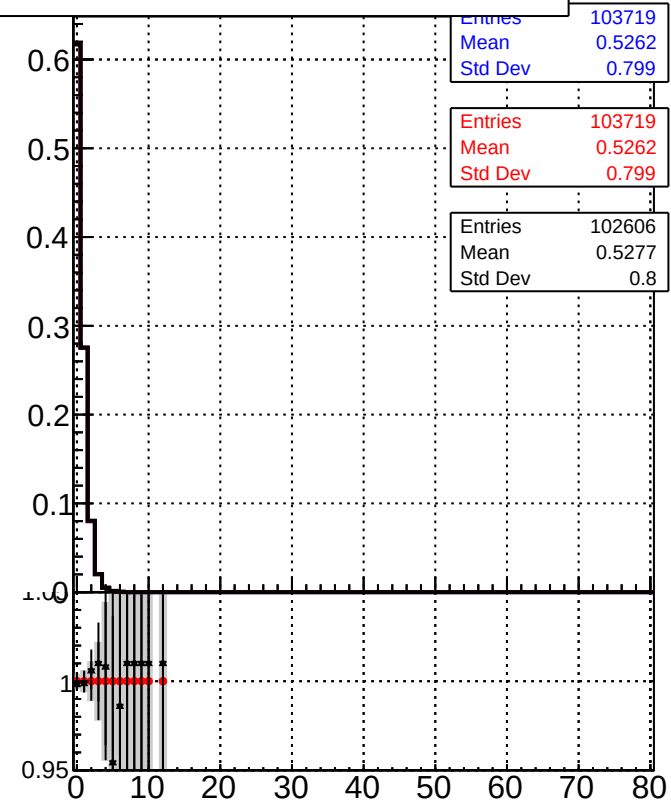
Legend: /data2/legianni/JSON-bkwd-fwd/no-modif/CMSSW_13_0_X_2023-01-24-1100/src/DQM_original (blue line with squares), DQM_modified (red line with circles), DQM_modified_4iter-NewERR (black line with crosses)
