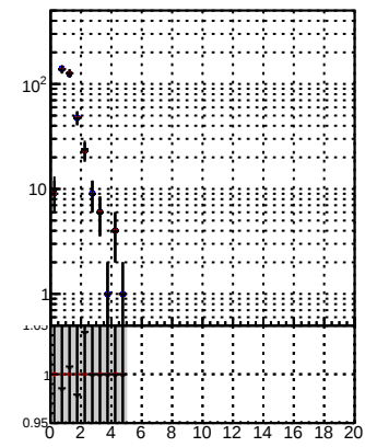
N of reco track vs. \chi^2 /data2/legion/j35N-bkwd-fwd/no-modif/CMSSW_13_0_X_2023-01-24-1100/src/DQM_modified_4iter-NewERR
