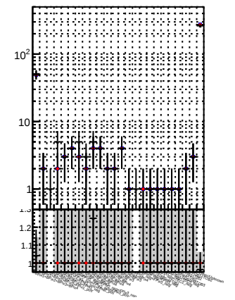
N of reco track vs. \chi^2 /data2/legion/j35N-bkwd-fwd/no-modif/CMSSW_13_0_X_2023-01-24-1100/src/DQM_modified_4iter-NewERR
