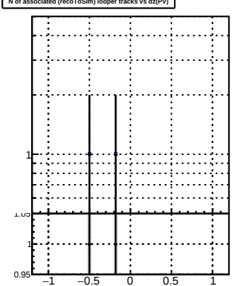
N of associated (recoToSim) loop tracks vs dz(PV)
