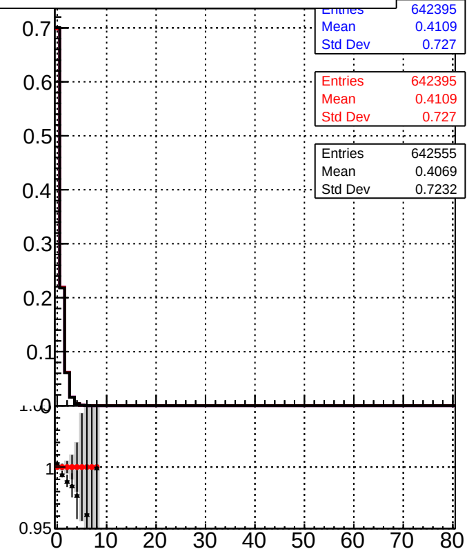
Legend for the bottom row of plots: —■— /data2/legianni/JSON-bkwd-fwd/no-modif/CMSSW_13_0_X_2023-01-24-1100/src/DQM_original —●— DQM_modified —+— DQM_modified_4iter-NewERR
