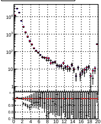
N of reco track vs. \chi^2 for data2/legsim/JSON-bkwd-fwd/no-modif/CMSSW_13_0_X_2023-01-24-1100/src/DQM_original and DQM_modified 4iter-NewERR
