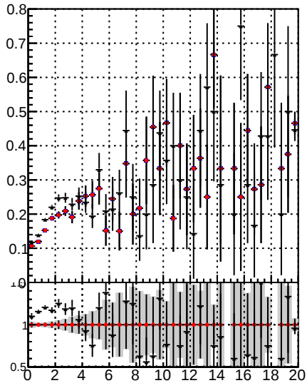
Fake rate vs. /data2/legianni/JSON-bkwd-fwd/no-modif/CMSSW_13_6_X_2023-01-24-1100/src/DQM_original BCM_modified_4iter-NewERR BCM_modified_4iter-NewERR
