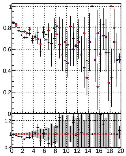
Fake rate vs. /data2/legianni/JSON-bkwd-fwd/no-modif/CMSSW_13_6_X_2023-01-24-1100/src/DQM_original BCM_modified_4iter-NewERR BCM_modified_4iter-NewERR
