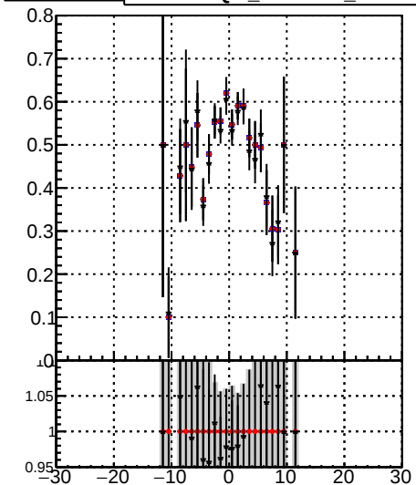
Fake rate vs vertpos /data2/legianni/JSON-bkwd-fwd/no-modif/CMSSW_13_0_X_2023-01-24-1100/src/DQM_original DQM_modified DQM_modified_4iter-NewERR
