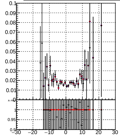
Efficiency vs vertpos Legend: \bullet /data2/legianni/JSON-bkwd-fwd/no-modif/CMSSW_13_0_X_2023-01-24-1100/src/DQM_original \bullet DQM_modified \bullet DQM_modified_4iter-NewERR
