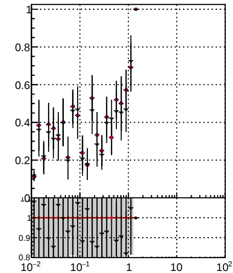
Fake rate vs vertpos Legend: \square /data2/legianni/JSON-bkwd-fwd/no-modif/CMSSW_13_0_X_2023-01-24-1100/src/DQM_original \bullet DQM_modified \times DQM_modified_4iter-NewERR
