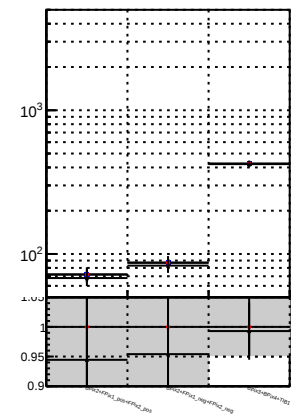
N of reco track vs. \chi^2 data2/legion/JSON-bkwd-fwd/no-modif/CMSSW_13_0_X_2023-01-24-1100/src/DQM_original DQM modified 4iter-NewERR
