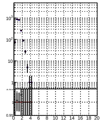
N of reco track vs. \chi^2 for JSON-bkwd-fwd-no-modif/CMSSW_13_0_X_2023-01-24-1100/src/DQM_original
