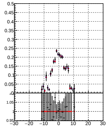
Legend: /data2/legianni/JSON-bkwd-fwd/no-modif/CMSSW_13_6_X_2023-01-24-1100/src/DQM_original (blue line), BQM modified 4iter-NewERR (red line), BQM modified 4iter-NewERR (black line)
