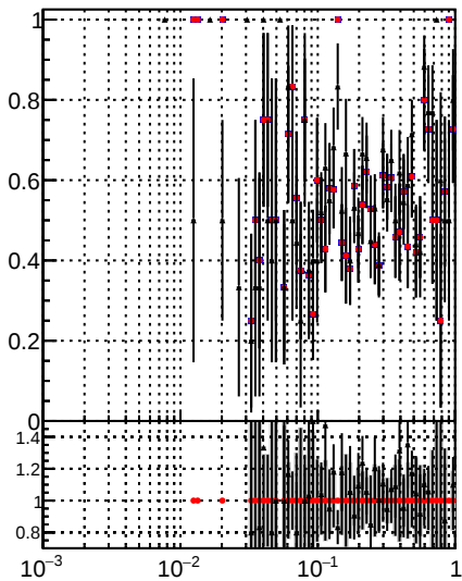
/data2/legianni/JSON-bkwd-fwd/no-modif/CMSSW_13_0_X_2023-01-24-1100/src/DQM_original Fake rate vs DQM_modified DQM_modified_4iter-NewERR
