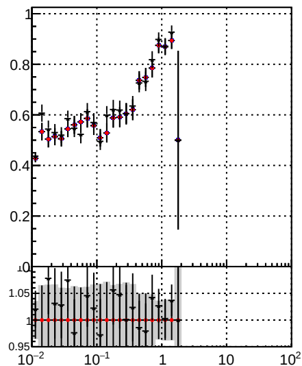
/data2/legianni/JSON-bkwd-fwd/no-modif/CMSSW_13_0_X_2023-01-24-1100/src/DQM_original Fake rate vs v DQM_modified Fake rate vs v DQM_modified_4iter-NewERR
